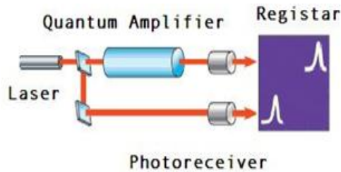
Figure 5. Experiments of L.Wang - superluminal light propagation.
