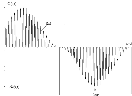
Figure 2. Behaviour of wave packet in linear dispersion medium
