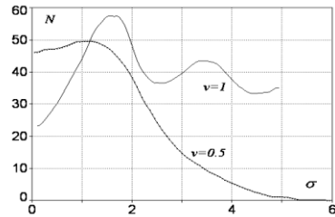
Fig.3.3. Dependence of particles number passed barrier on barrier width \sigma for different velocities.
