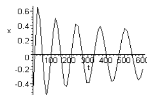
Fig.5.6. "Crematorium" solution.
