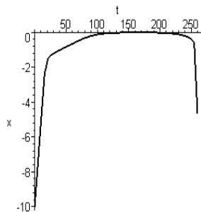
Fig.3.5. Reflection from barrier with increased velocity.
