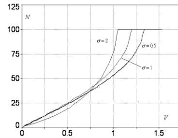
Fig.3.4. Dependence of barrier transparency on velocity for different barrier width.
