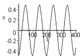
Fig.5.5. Classical solution.
