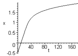
Fig.5.2. "Crematorium" solution.
