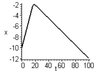
Fig. 3.7. Reflection from barrier with loss of velocity.
