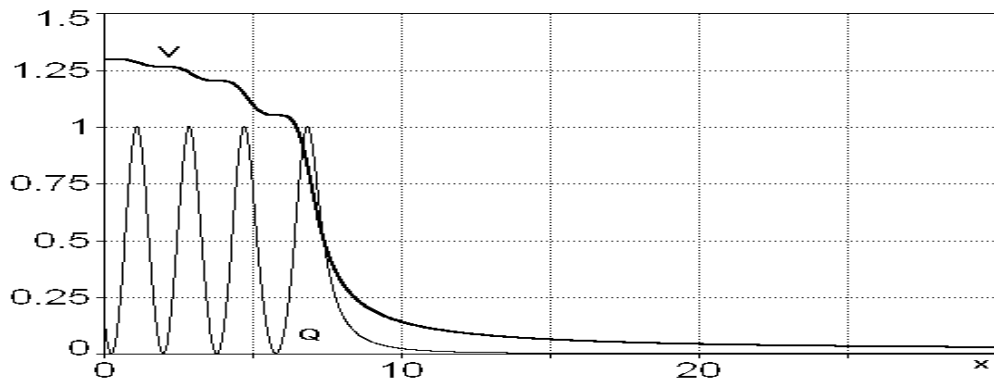
Fig.2.3 Dependence of particle's velocity and its charge on distance from barrier.
