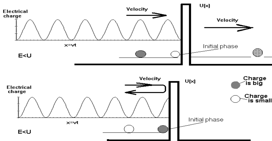
Fig.2.3 Dependence of particle's velocity and its charge on distance from barrier.
