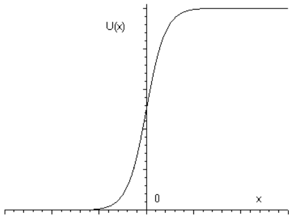
Fig. 2.1 The step's potential U(x) .
