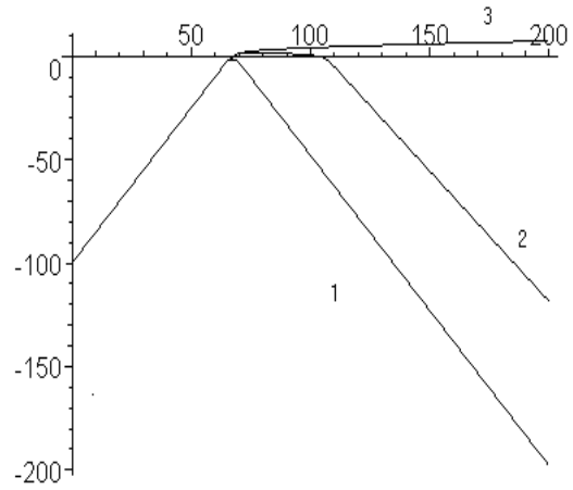
Fig.2.2 Reflection (1 and 2) and passage (3) of particles with different values of initial phase.
