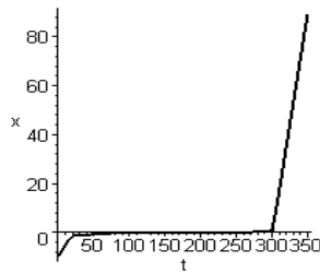
Fig. 3.6. Passing of barrier with increased velocity .
