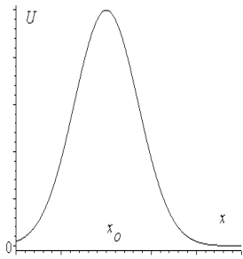
Fig.3.2. Potential barrier .
